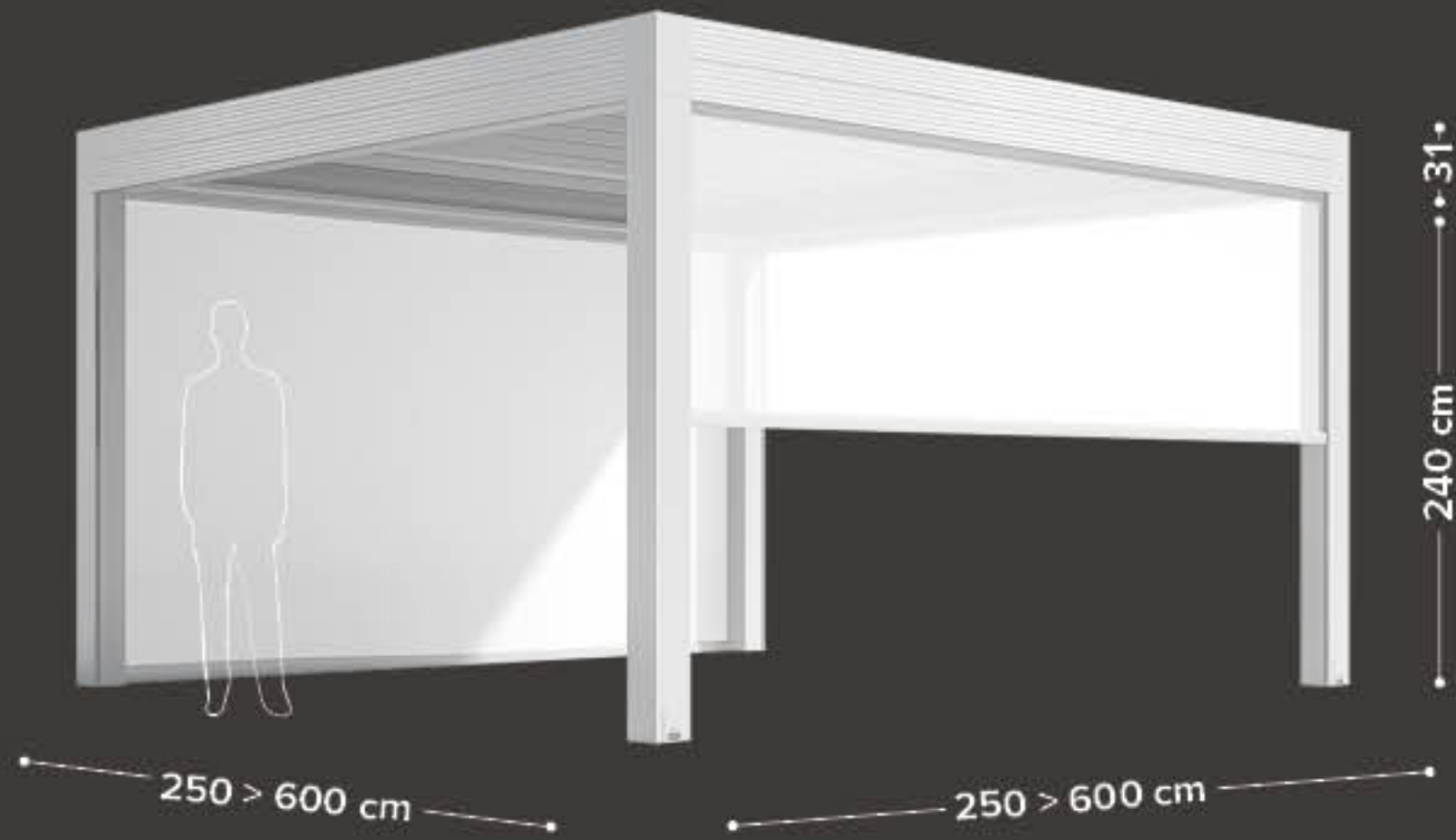
ISOLA / ISLAND monomodulo 4 gambe basic module 4 posts
